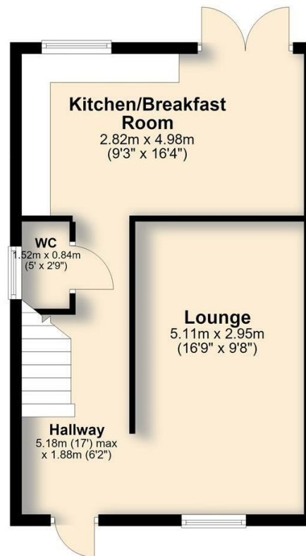
Ground Floor Approx. 39.7 sq. metres (427.0 sq. feet)
